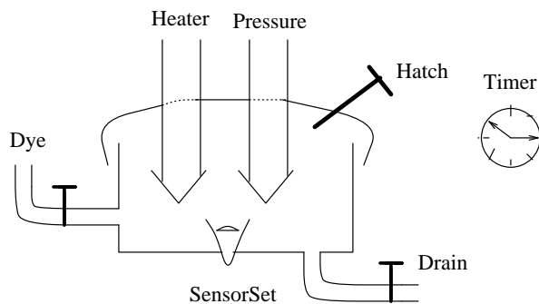
Figure 3: Dyeing Machine
