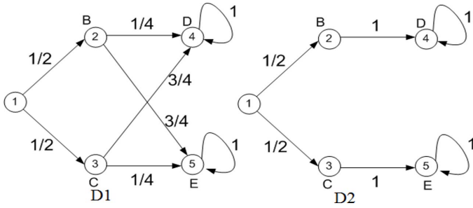
Fig. 1. Discrete Time Markov Chains distinguishable by PCTL* formula.
